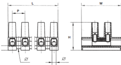
CTSN433/12LC larger isolating surface per pole and screw tower. Complies with EN60598/1 4.7 and 11.2
