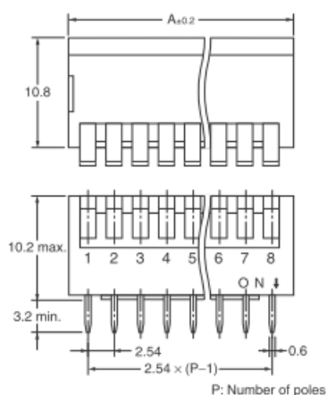
Short actuator
