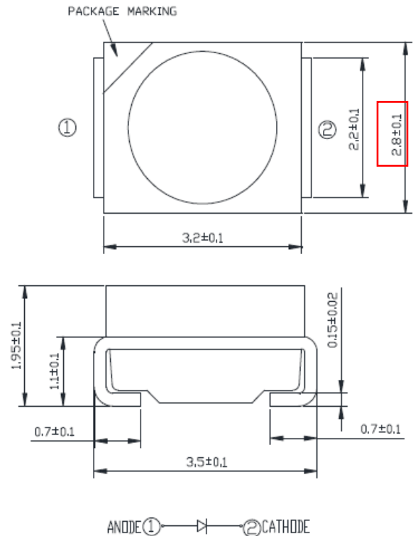
New dimension drawing
