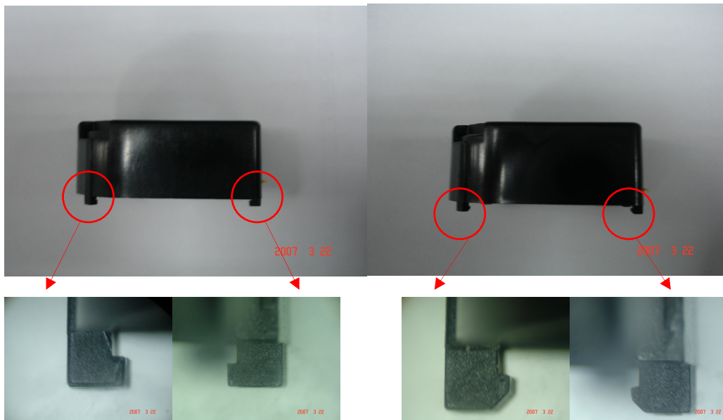
Existing latch
