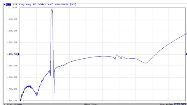
S21 (Broadband)
