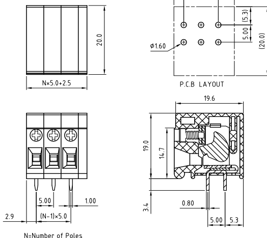
Drilling Diagram & Footprint (top view)
