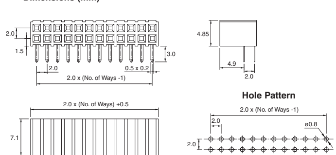
Dimensions (mm)
