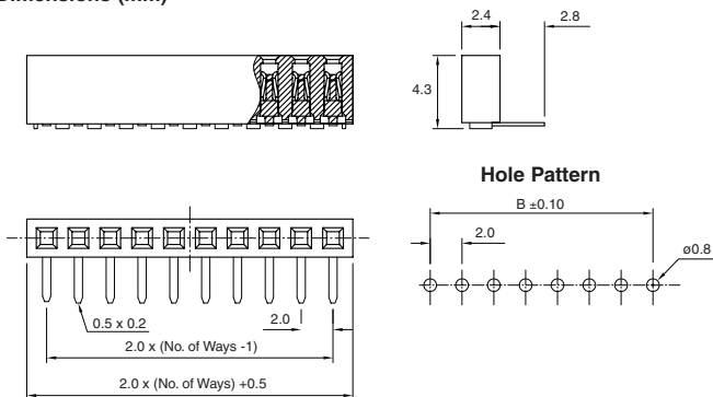
Dimensions (mm)
