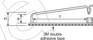
Dimensions (mm)
